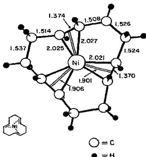
Fig. 30. A perspective drawing of all- trans -1,5,9 cyclododecatrienickel(0). Adapted with permission from ref. 269.
