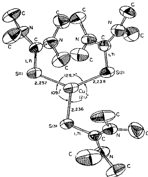
Fig. 18. The structure of [Cu(tmtu)_3]^+ showing the non-symmetrical arrangement of the tetramethylthiourea ligands around copper. Reproduced with permission from ref. 187.
