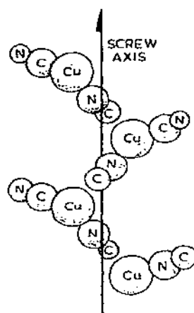
Fig. 25. A drawing of the [\text{Cu}(\text{CN})_2]_\infty polymer chain. The view is normal to y at an angle such that all of the copper atoms are in the plane of the paper. Adapted with permission from ref. 215.
