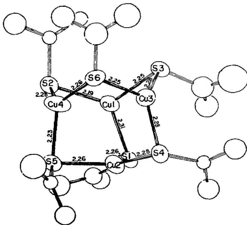
Fig. 23. A perspective drawing of the [\text{Cu}_4(\text{tu})_6]^{4+} cluster, which has an adamantane-like structure similar to that in [\text{Cu}_4(\text{tu})_9]^{6+} . However, in the [\text{Cu}_4(\text{tu})_6]^{4+} cluster each copper atom is three-coordinate. Published with permission of E.L. Amma, ref. 194.
