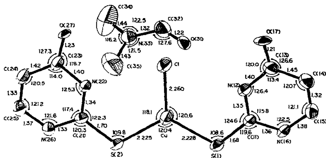
Fig. 24. An ORTEP drawing of the chloro-bis(2-thiouracil)copper(I) molecule and of a dimethylformamide molecule of solvation. Reproduced with permission from ref. 208.
