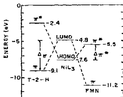
Fig. 11. Energy level diagram showing the relative positions of the highest occupied and lowest unoccupied MO's of \text{Ni}[\text{P}(\text{O}-o\text{-tolyl})_3]_3 , trans -2-hexene (T-2-H) and fumaronitrile (FMN). Reproduced with permission from ref. 87.
